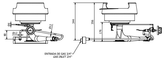
ENTRADA DE GAS 3/4" GAS INLET 3/4"
