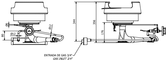
ENTRADA DE GAS 3/4" GAS INLET 3/4"
